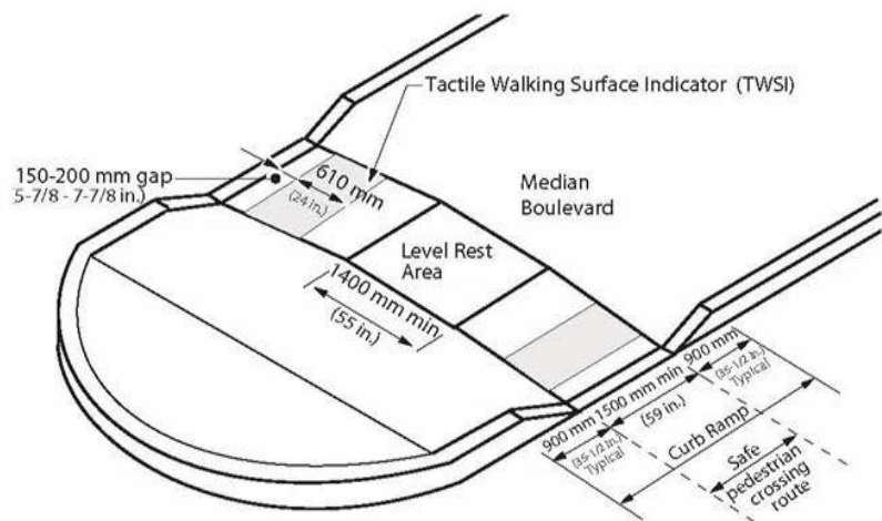
Figure 4.1.10.4 Curb Ramp at Wide Median Sidewalk Crossing
