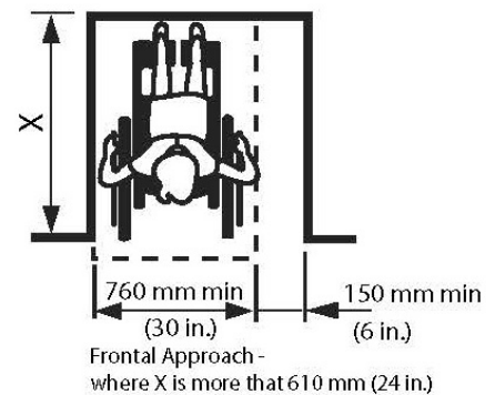
Figure 4.1.1.8 Clearances at Alcove
