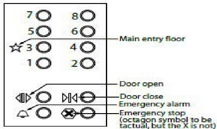
Figure 4.1.14.4 Tactile Symbols
