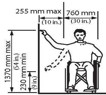
Figure 4.1.1.9 Side Reach
