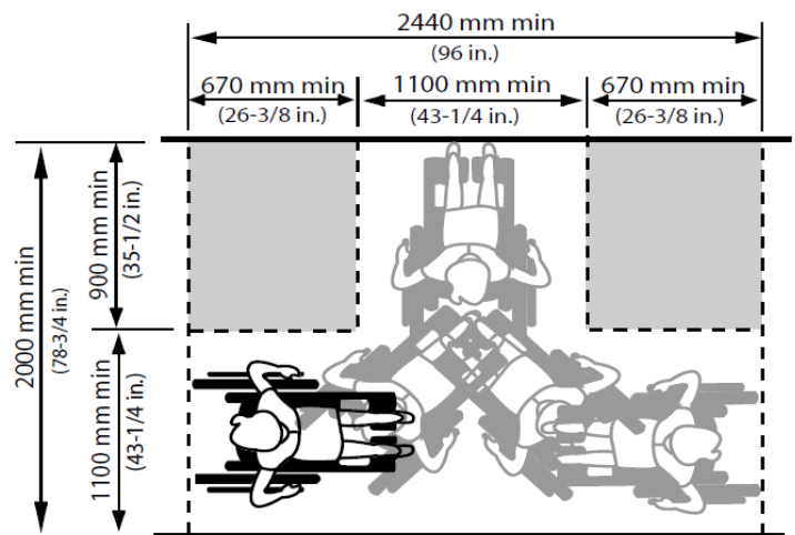
Figure 4.1.1.2 180° Turning Space
