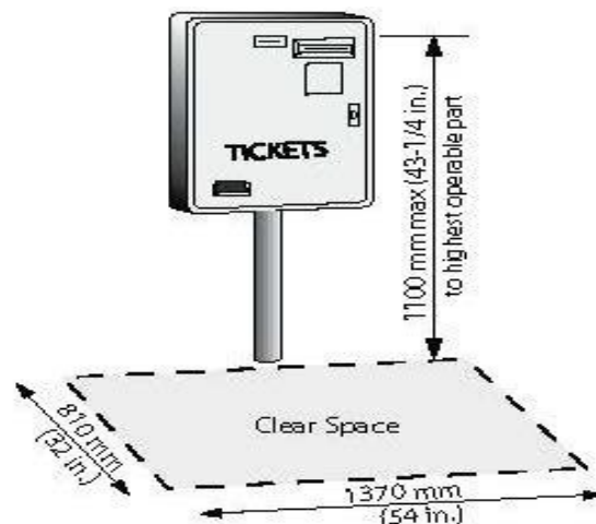
Figure 4.4.3.2 Ticket Dispensing Machine
