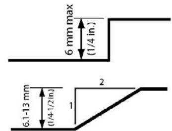
Figure 4.1.2.1 Changes in Level
