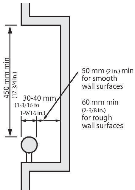
Figure 4.1.12.3 Handrail in Recess
