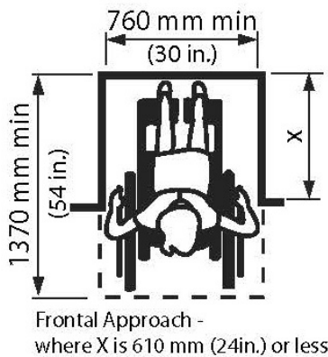
Figure 4.1.1.7 Clearances at Alcove
