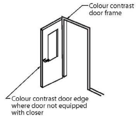
Figure 4.1.6.9 Colour Contrast at Doors
