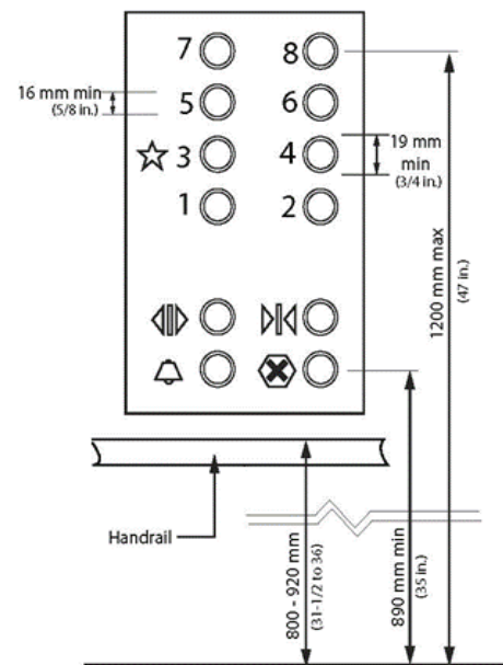
Figure 4.1.14.2 Control Panel
