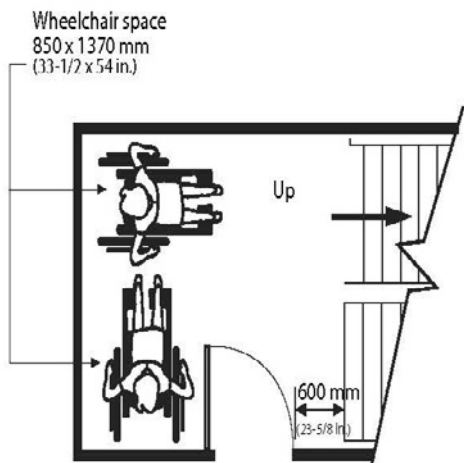
Figure 4.4.1.1 Area of Rescue Assistance
