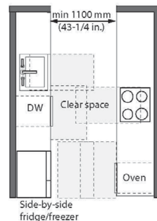
Figure 4.3.18.1 Pass-Through Kitchen
