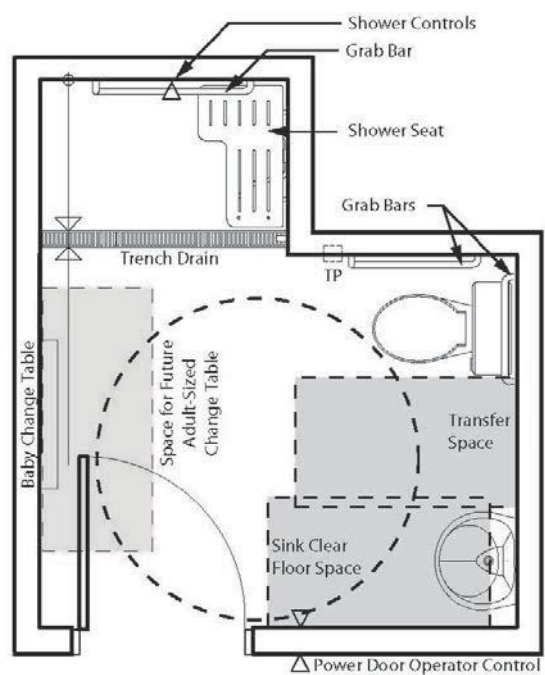
Figure 4.5.7.2 Universal Washroom - New Construction
