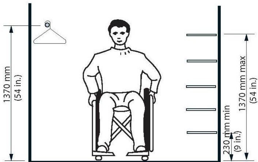
Figure 4.3.9.1 Reach Limits for Storage
