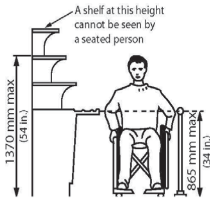
Figure 4.5.4.1 Self Serve Counter
