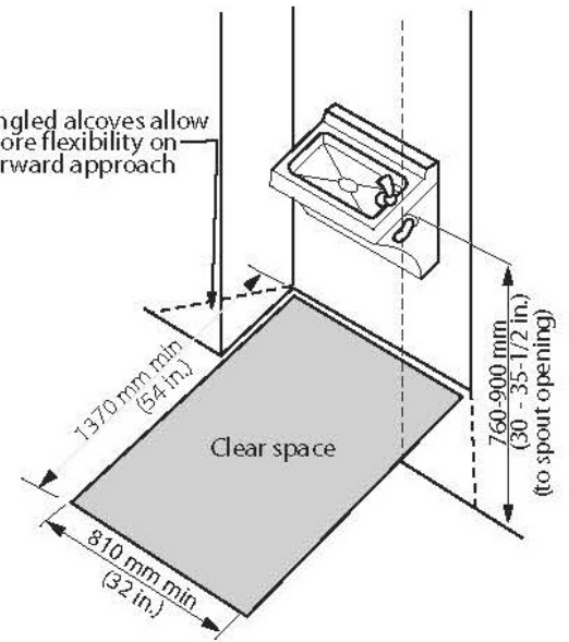
Figure 4.3.1.2 Forward Approach
