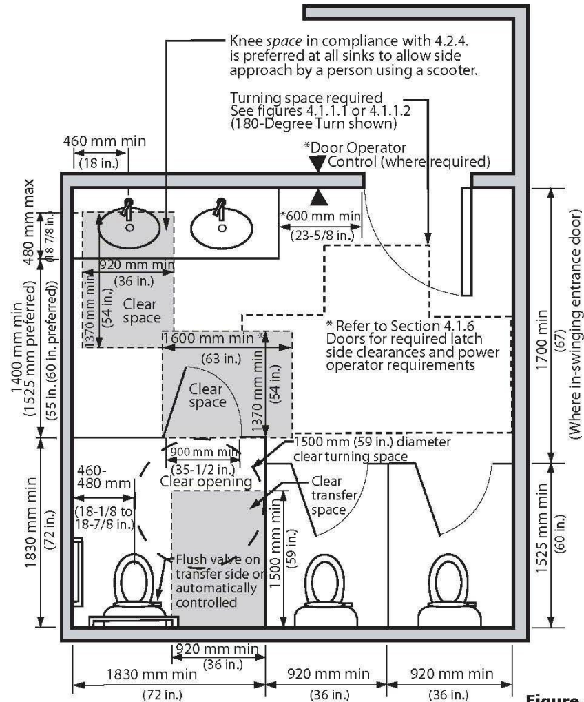
Figure 4.2.1.1 Washroom Dimensions
