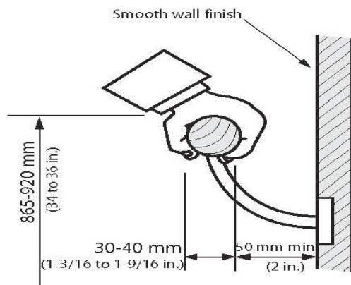
Figure 4.1.12.1 Handrail
