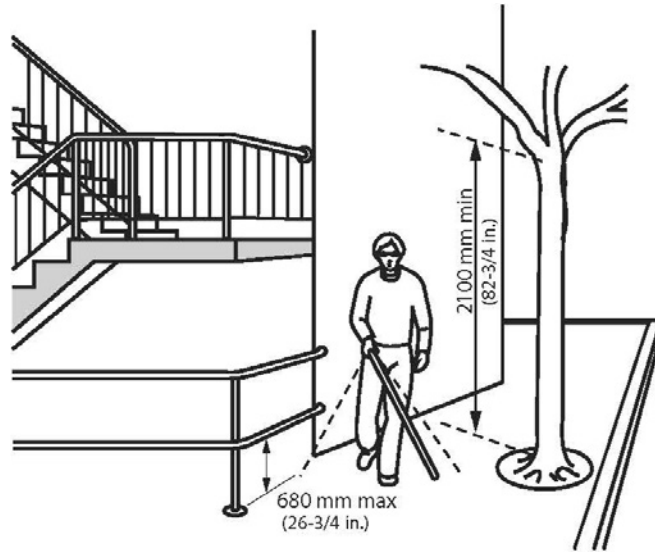
Figure 4.1.3.3 Overhead Obstructions
