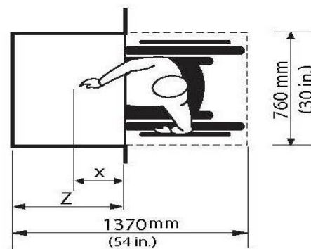
Figure 4.1.1.14 Forward Reach over an Obstruction
