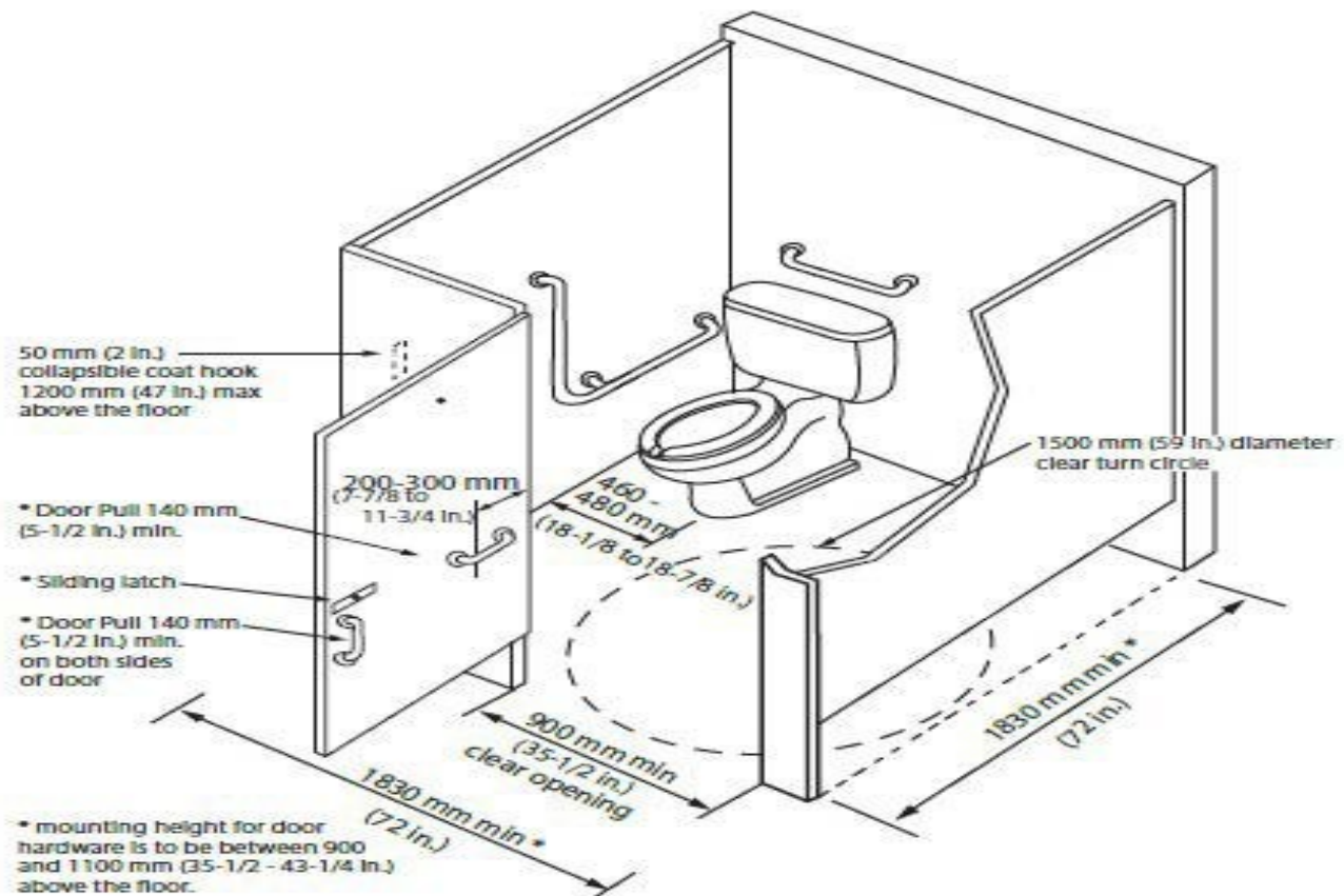
Figure 4.2.2.1 Accessible Toilet Stall
