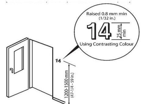
Figure 4.4.7.3 Tactile Lettering
