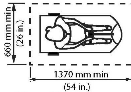
Figure 4.1.1.6 Clear Floor Space for Scooter
