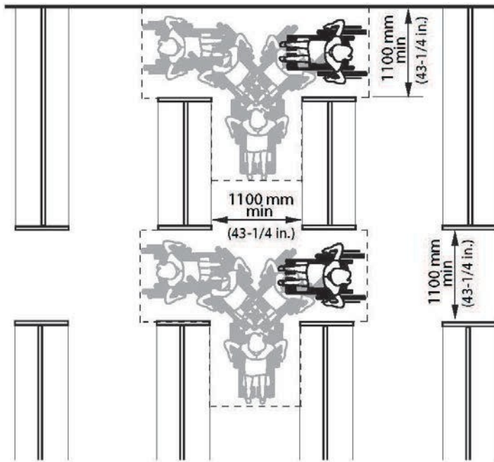
Figure 4.5.5.1 Aisle Width
