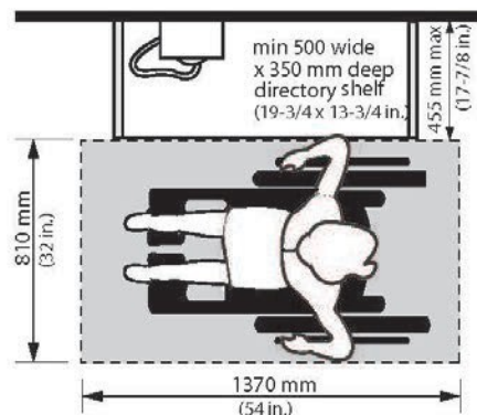
Figure 4.4.5.3 Parallel Approach to a Public Telephone
