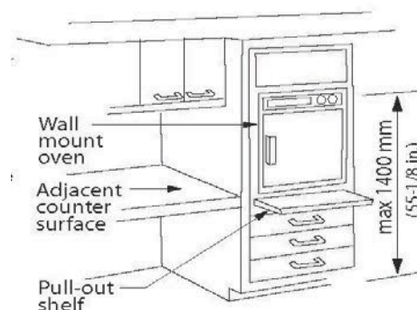
Figure 4.3.18.8 Wall-Mounted Oven
