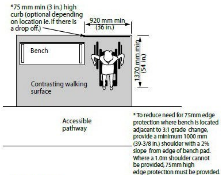
Figure 4.3.15.1 Rest Area
