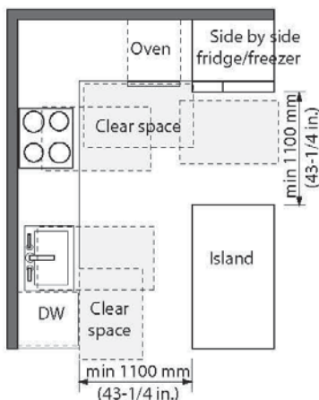
Figure 4.3.18.3 L-Shaped Kitchen with Island
