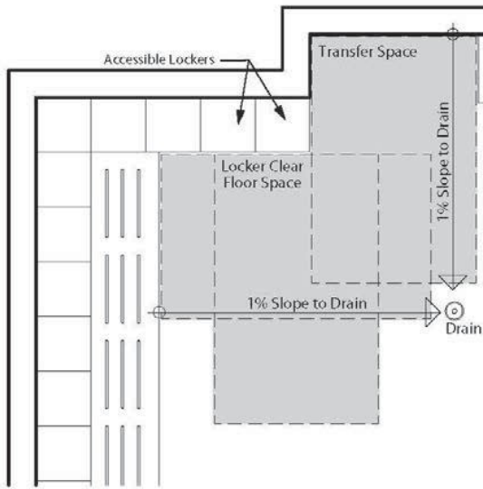
Figure 4.3.10.1 Locker Room Clear Floor Space requirements
