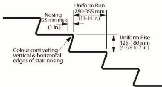
Figure 4.1.11.2 Stair Tread Criteria
