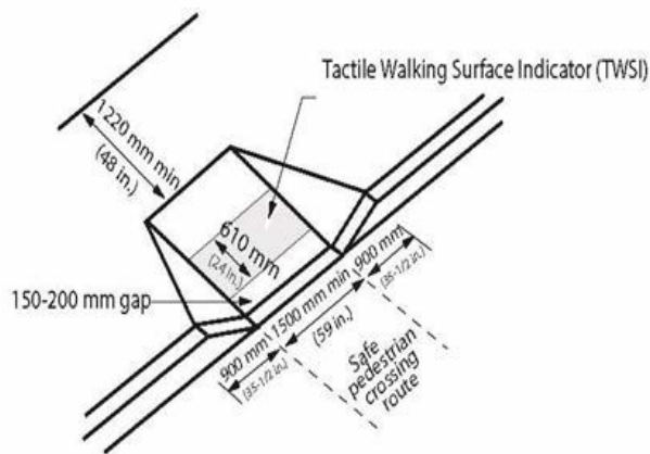
Figure 4.1.10.6 Curb Ramp at Mid-Block Crossing (refer also to Ontario Provincial Standards for Roads & Public Works (OPSD))
