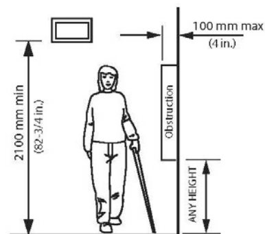
Figure 4.1.3.2 Limits of Protruding Objects
