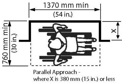
Figure 4.1.1.3 Clearances at Alcove
