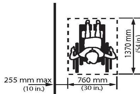
Figure 4.1.1.13 Side Reach - Maximum Distance to Wheelchair
