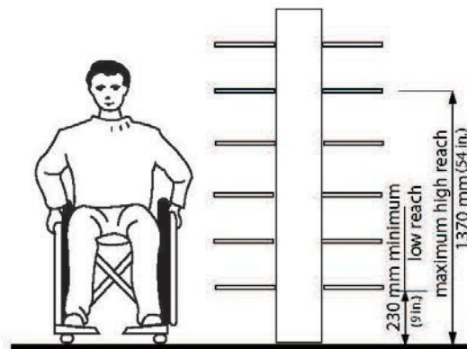
Figure 4.5.5.2 Reach Heights
