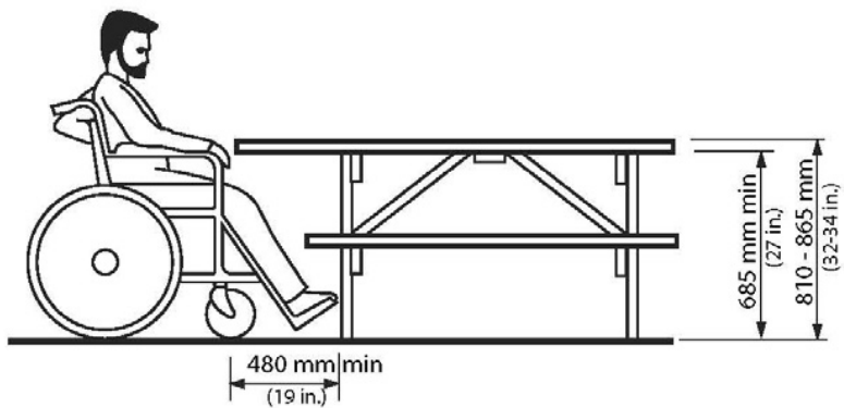
Figure 4.3.16.1 Height and Knee Space at Accessible Tables
