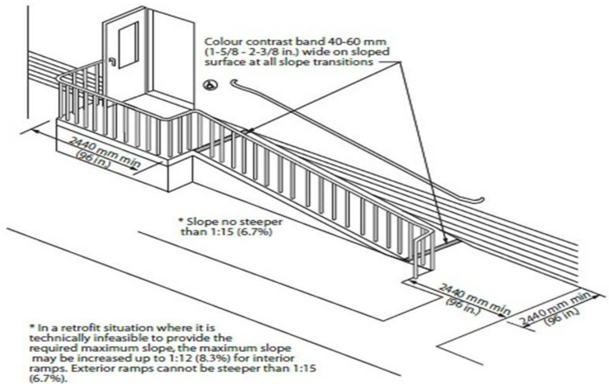
Figure 4.1.9.2 Ramp Criteria
