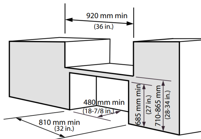
Figure 4.3.8.1 Service Counter
