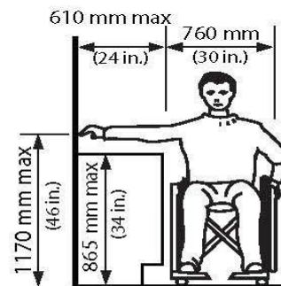
Figure 4.1.1.10 Side Reach over an Obstruction
