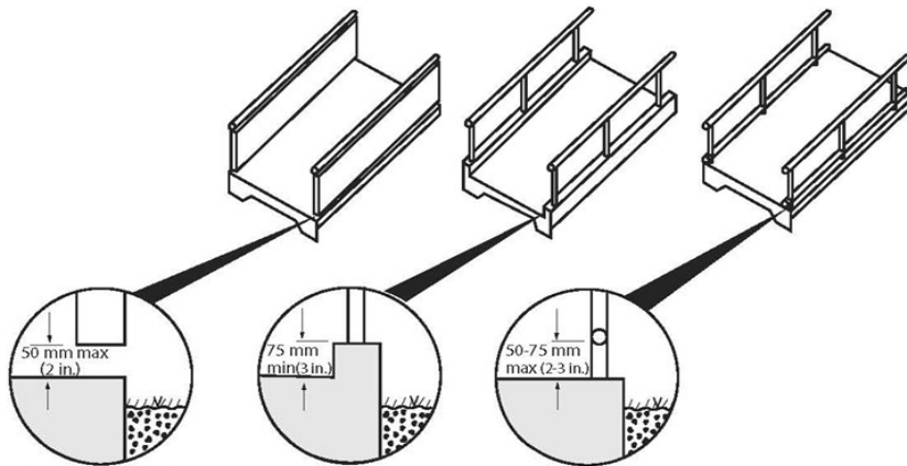
Figure 4.1.9.4 Edge Protection at Ramps
