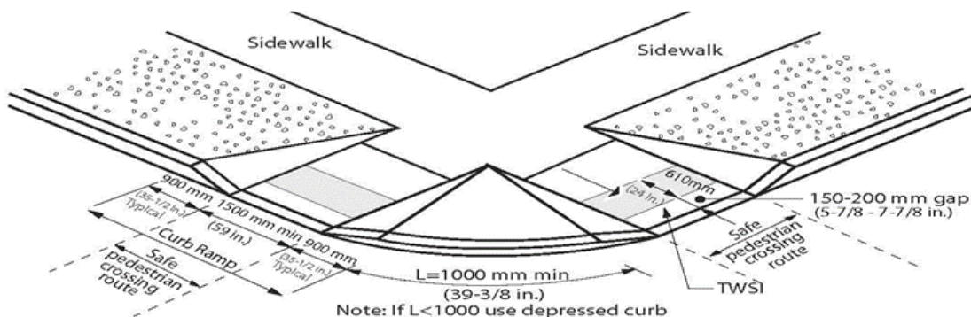
Figure 4.1.10.1 Standard Curb Ramp
