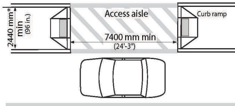
Figure 4.3.13.3 Alternate Passenger Loading Zone Configuration
