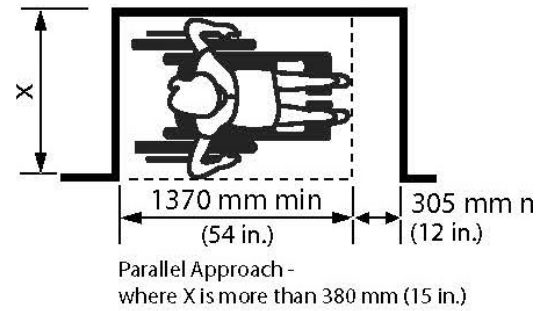
Figure 4.1.1.4 Clearances at Alcove
