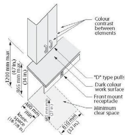
Figure 4.3.18.4 Storage Elements
