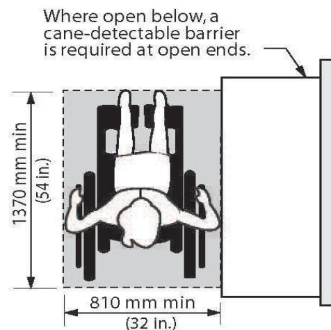
Figure 4.3.7.3 Parallel Approach
