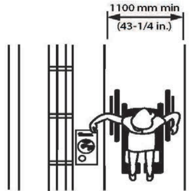
Figure 4.5.4.2 Aisle Width
