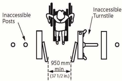
Figure 4.1.7.1 Access at Turnstile
