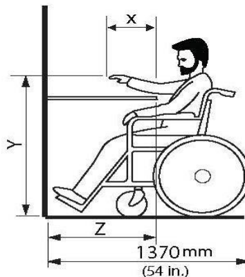
Figure 4.1.1.12 Forward Reach over an Obstruction
