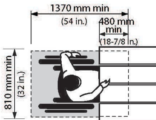
Figure 4.3.7.2 Frontal Approach
