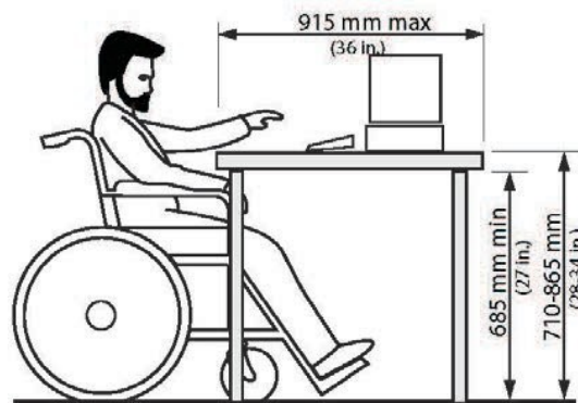
Figure 4.5.5.3 Work Surfaces
