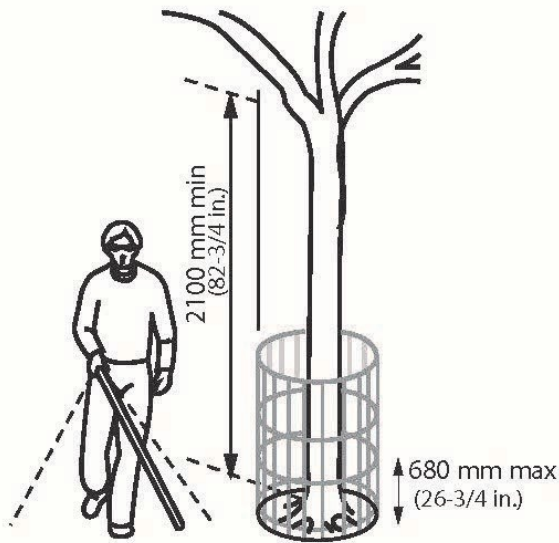
Figure 4.3.14.1 Tree Guard
