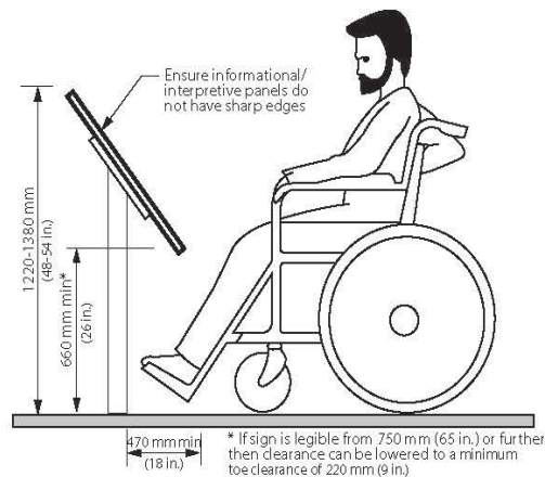
Figure 4.4.10.1 Critical dimensions for information systems and displays
