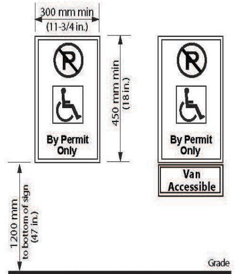
Figure 4.3.12.3 Regulatory Parking Signage
