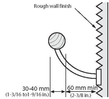
Figure 4.1.12.2 Handrail at Rough Wall
