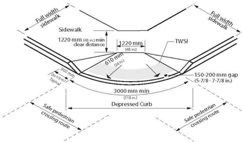
Figure 4.1.10.2 Alternate Curb Ramp for situations where figure 4.1.10.1 is not feasible.
