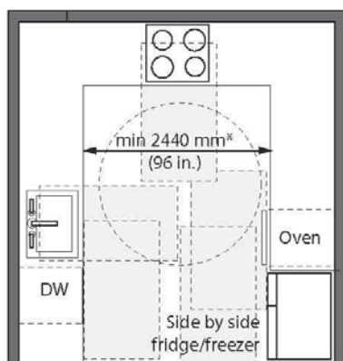
Figure 4.3.18.2 U-Shaped Kitchen
