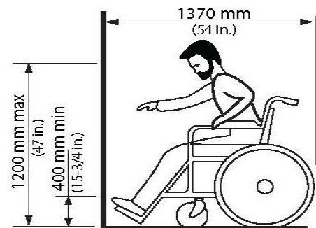
Figure 4.1.1.11 Forward Reach
