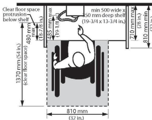
Figure 4.4.5.4 Forward Approach to a Public Telephone
