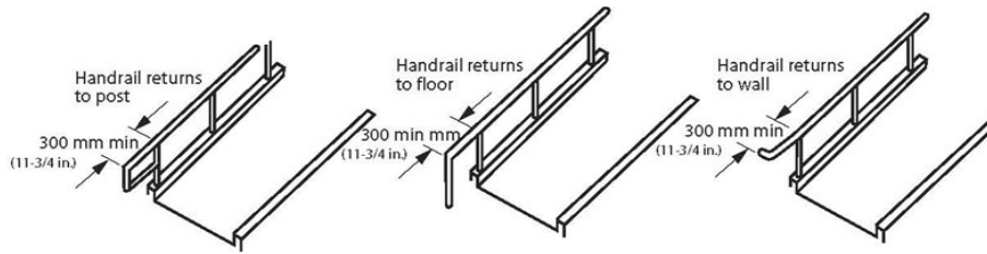
Figure 4.1.9.3 Horizontal Handrail Extensions
