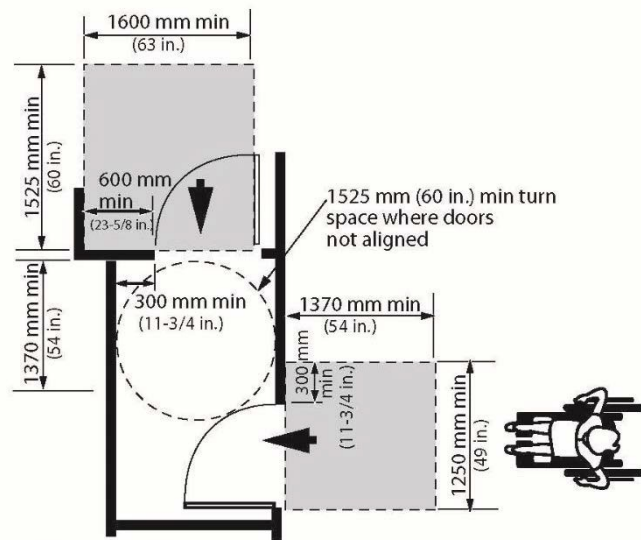
Figure 4.1.6.6 Manoeuvring Space at Doors in Series
