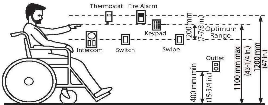
Figure 4.4.2.1 Reach Range for Accessible Controls
