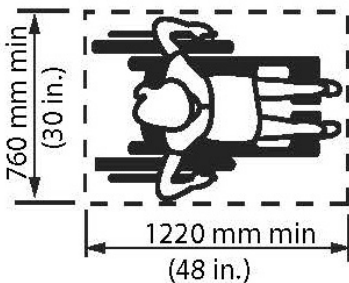
Figure 4.1.1.5 Clear Floor Space for Wheelchair
