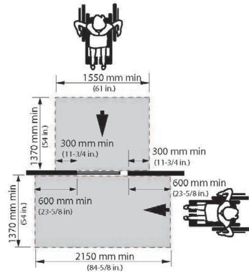
Figure 4.1.6.4 Front and Side Approach at Sliding Doors
