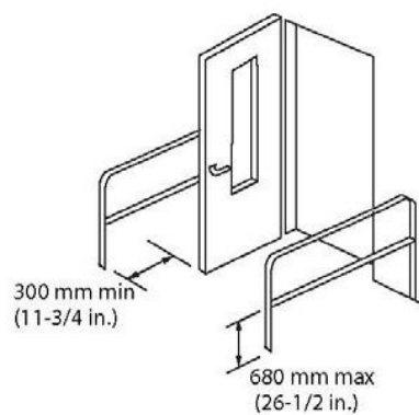
Figure 4.1.6.8 Detectable Safety Guards
