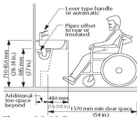
Figure 4.3.18.5 Kitchen Sink
