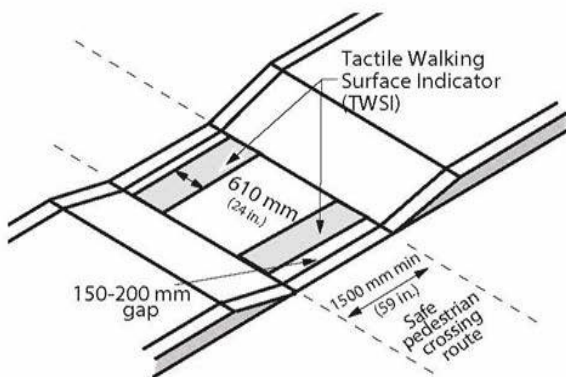
Figure 4.1.10.3 Curb Ramp at Narrow Median Sidewalk Crossing
