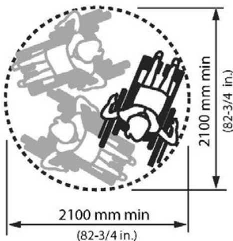
Figure 4.1.1.1 360° Turning Space
