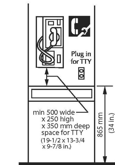
Figure 4.4.5.2 Accessible Telephone for Persons who are Deaf, Deafened, Hard of Hearing, or Speech-Impaired
