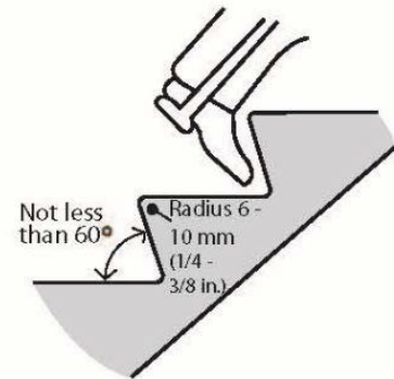
Figure 4.1.11.3 Raked Riser
