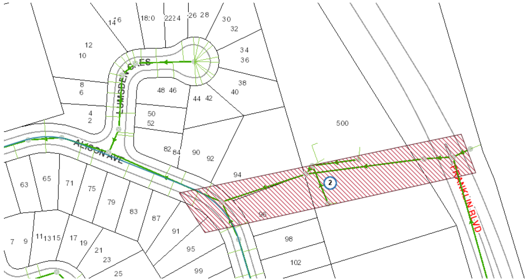
Fig 2 Alison Ave.-Franklin Blvd. (Utility Corridor)500 Franklin Blvd. Sanitary Sewer
