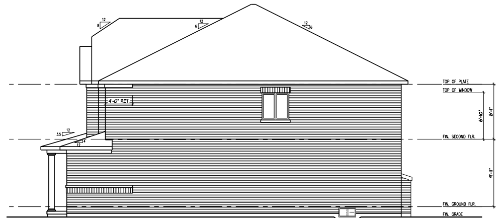
RIGHT SIDE ELEVATION 'B'
