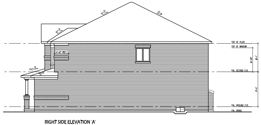
Proposed 2-Storey Elevations - Elevation A Source: Davide Cirocco (March 2020)
