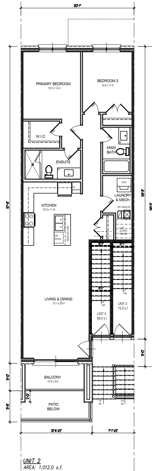
2nd LEVEL FLOOR PLAN
