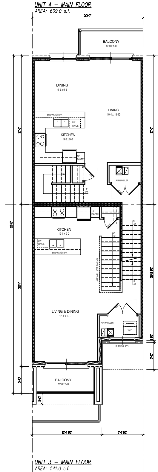
3rd LEVEL FLOOR PLAN
