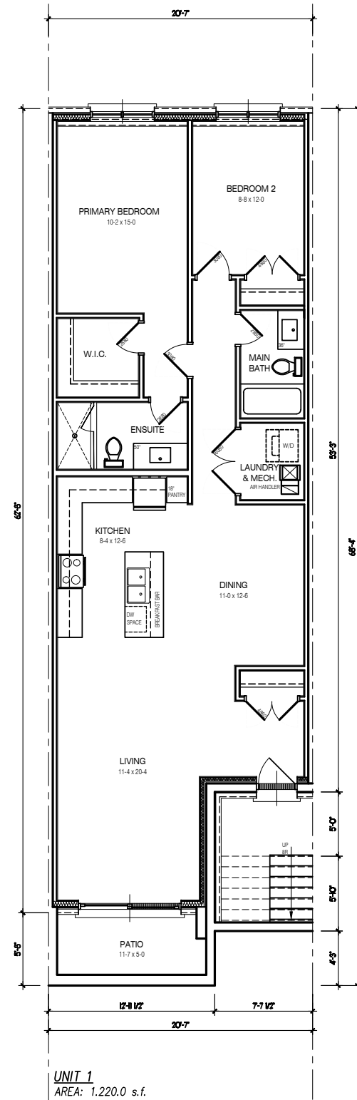
1st LEVEL FLOOR PLAN
