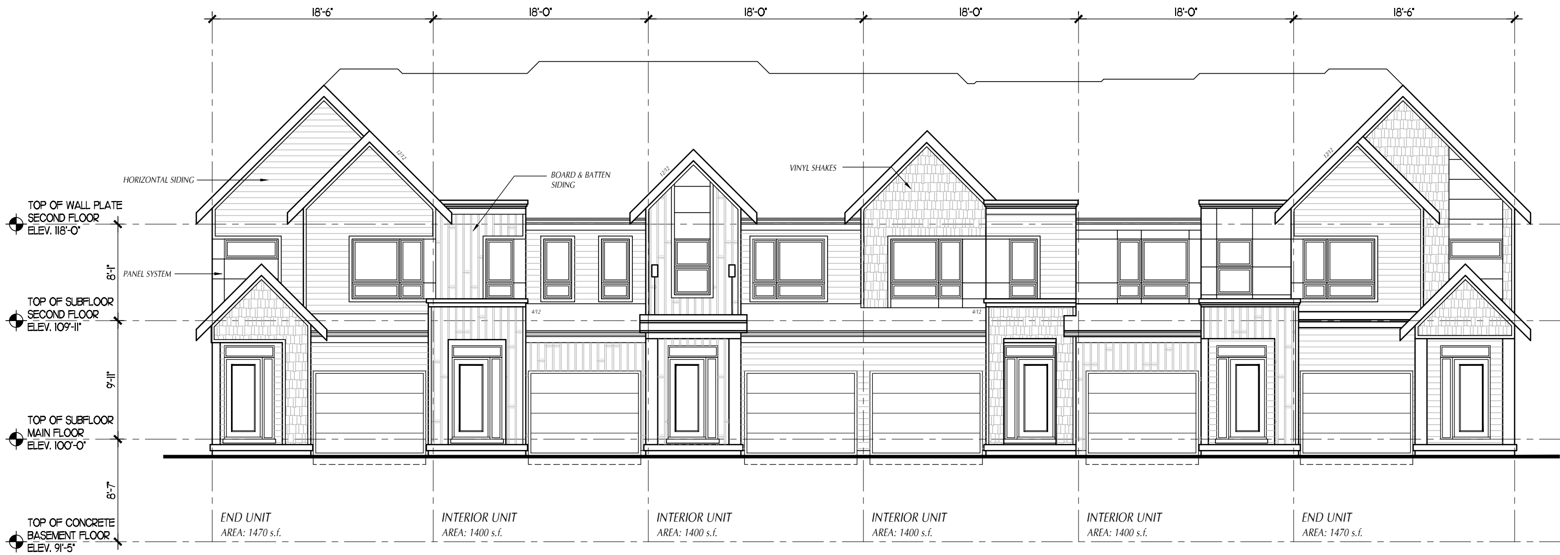
BLOCK FRONT ELEVATION
